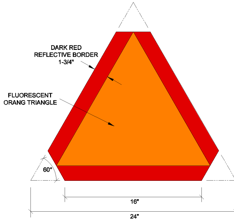
SLOW MOVING VEHICLE FACE
